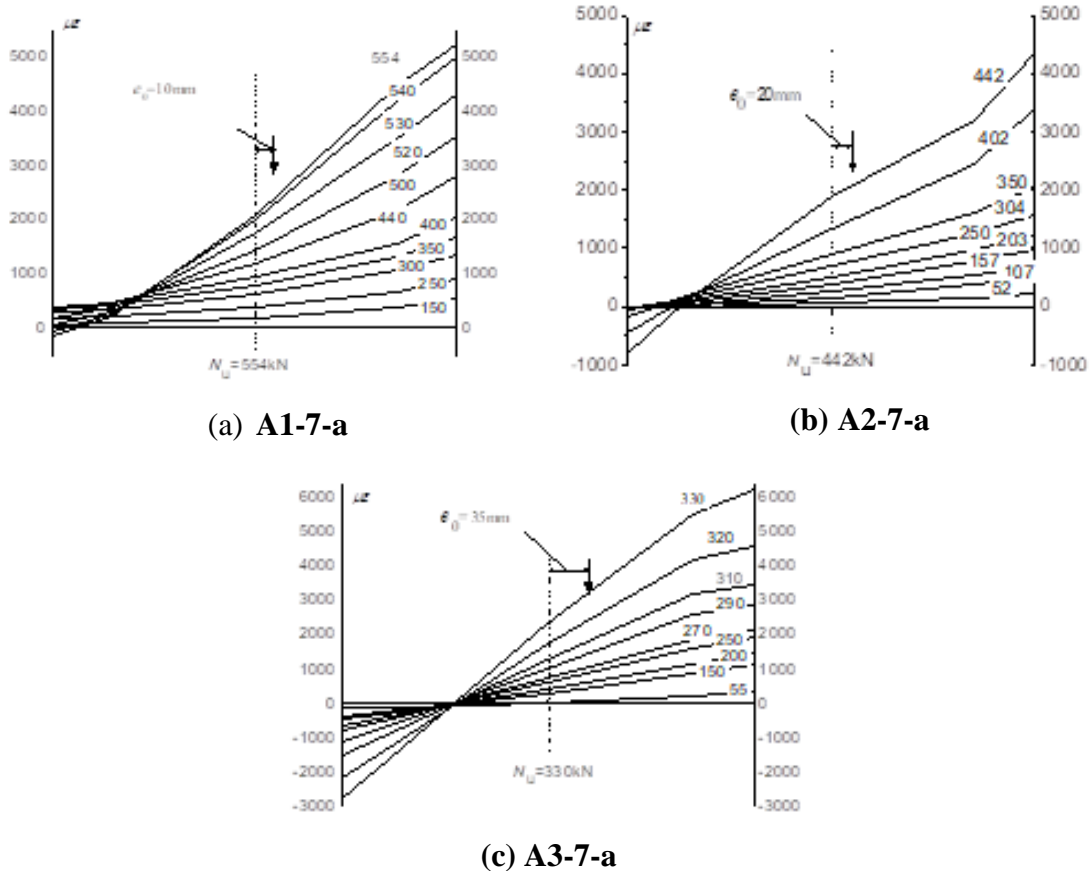
Figure 4: Distribution of Strain Due to Different Eccentric Ratios
